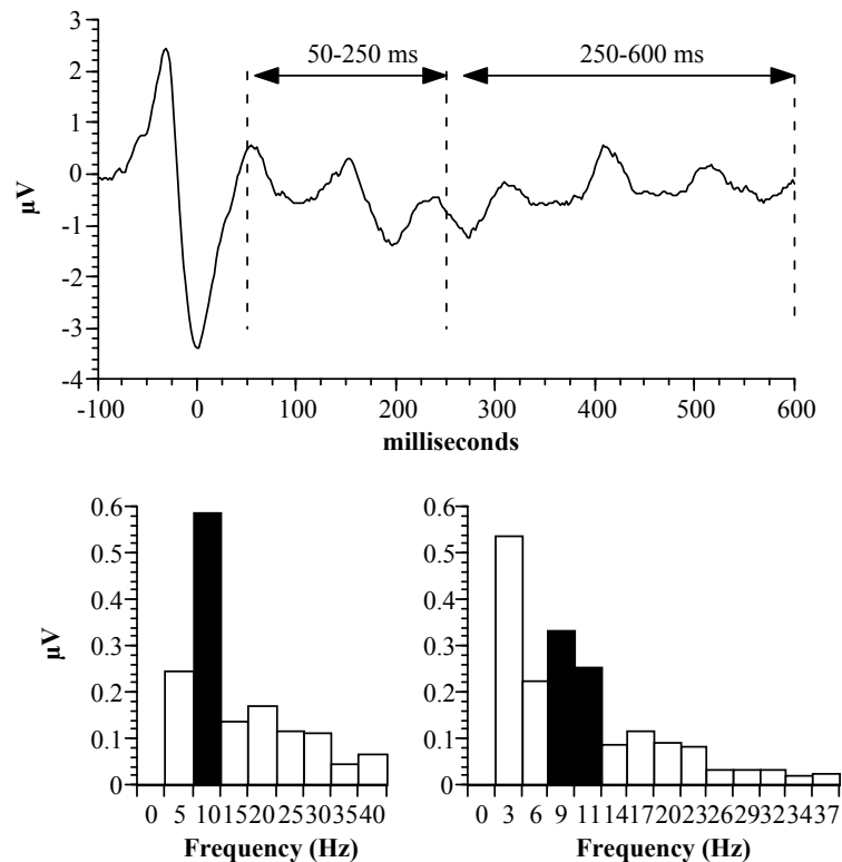
Figure 21. Quantification of alpha rhythm–ECG synchronization. In order to quantify the amount of alpha activity that is synchronized to the heart, a spectral analysis of the heartbeat evoked potential waveforms is performed. In this example the waveform is divided into two segments that represent different physiological mechanisms. The segment between 50–250 milliseconds reflects the processing of afferent signals, while the segment between 250–600 milliseconds reflects a combination of afferent processing and effects of the blood pressure wave reaching the brain.
