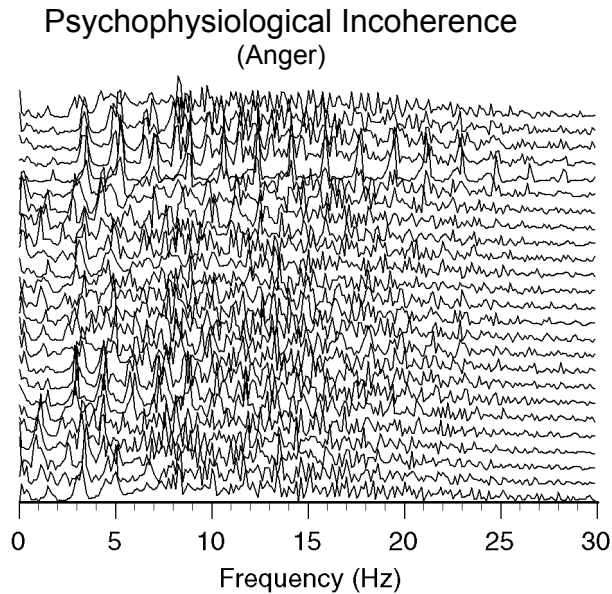
Figure 29. Waterfall plot of ECG spectra for the Psychophysiological Incoherence mode. In this example, anger is used to illustrate the mode, although most negative emotions also lead to incoherence. Note the lack of a coherent structure from spectrum to spectrum and the absence of harmonics in the spectra.
